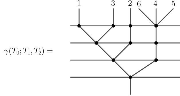
Figure 6: Partial compositions of the family represented in Figure 5.
