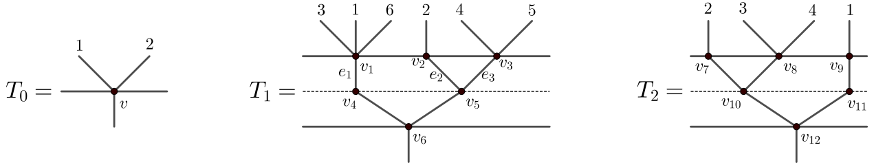
Figure 11: Example of family of leveled trees with k = 2 .
